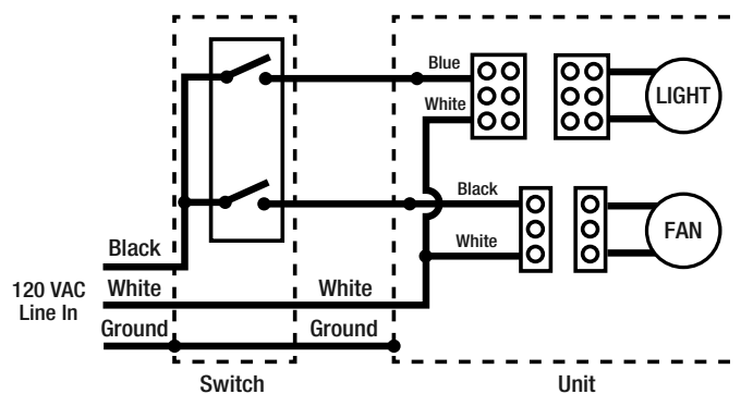
TO CONTROL FAN AND LIGHT INDEPENDENTLY
