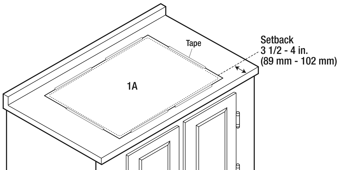
Topmount installation
